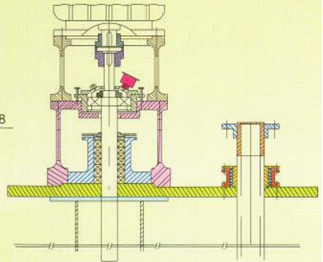
Pumps with Vapour Sealing arrangement.
